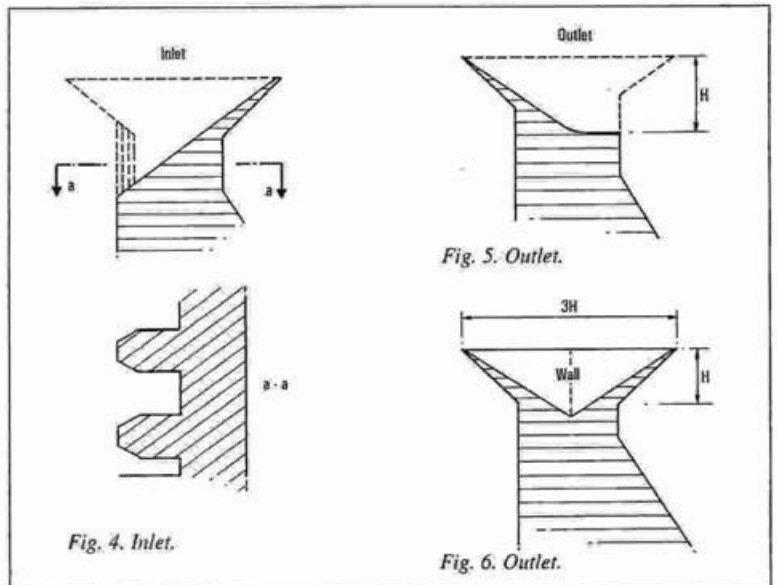
Figs. 4, 5 and 6. Variations to the hydraulic shape of the inlet and outlet.
