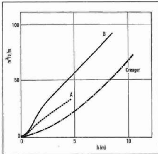
Fig. 3. Data for a wall height of 8 m.
