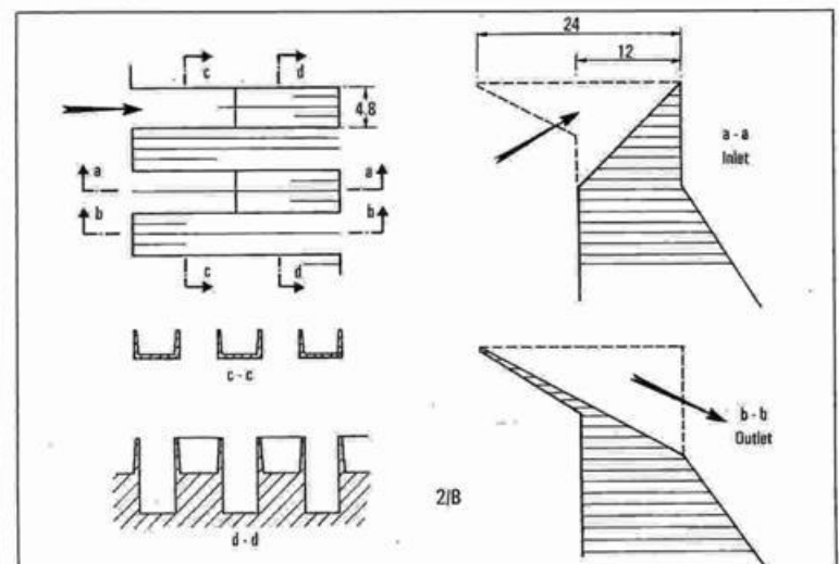
Fig. 2. The layout for Model B.
