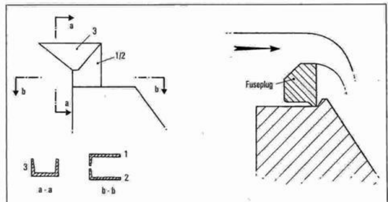
Fig. 7 (below left): construction using pre-cast elements. Fig. 8 (below): the use of a fuseplug to increase spillway capacity.
